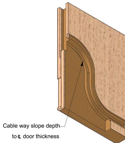
Door Core mortice through Lead Cover hung side Detail
