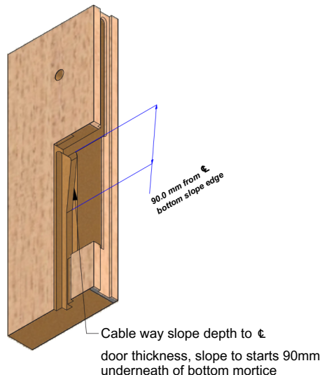
Door Core mortice through Lock lead side Detail
