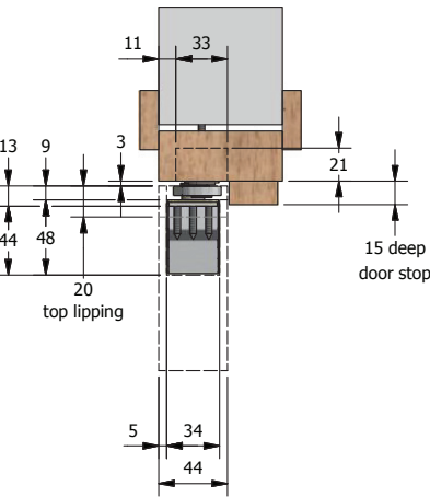
Vertical Section
