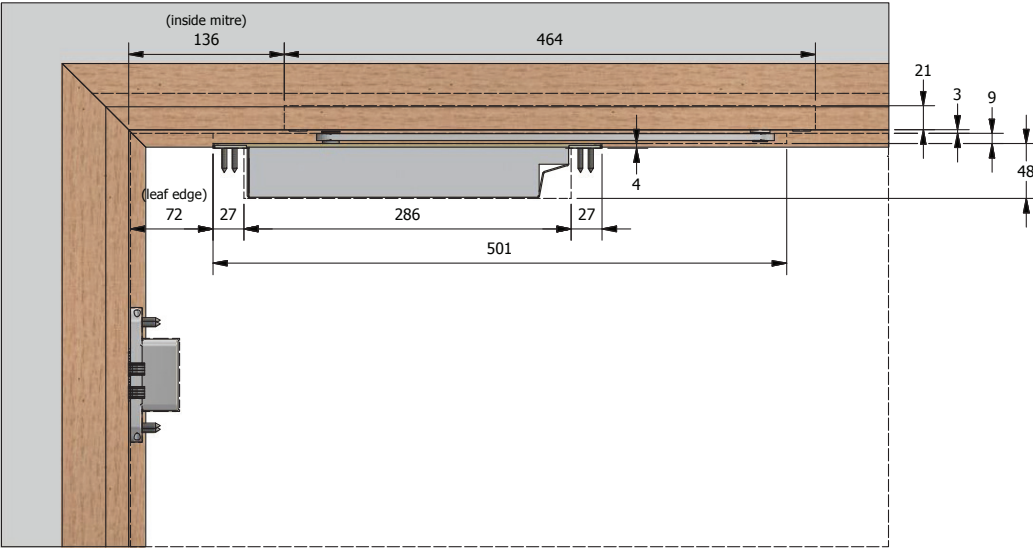
Vertical Section
