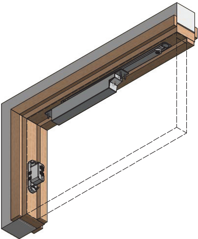
Isometric - Door Head
