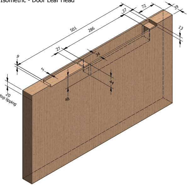
Isometric - Door Leaf Head
