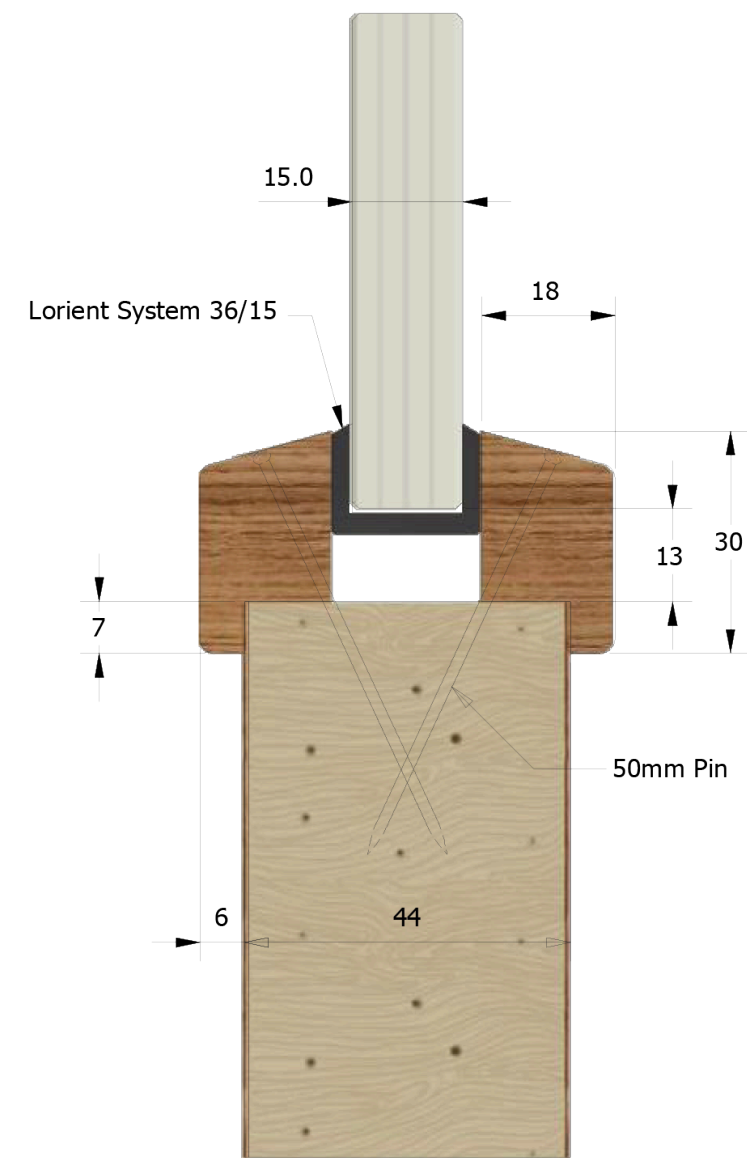
15mm Pyrostop FD30/30 (G60/8)
