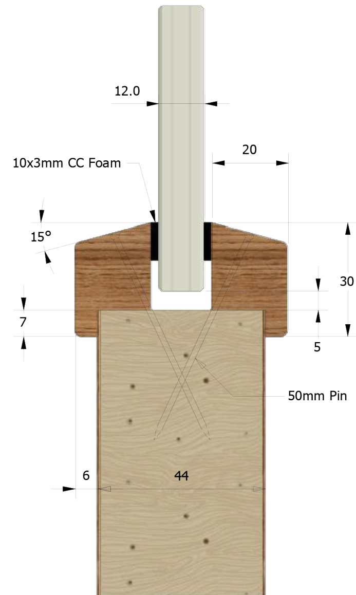
12mm Fire Laminate FD30/0 (G60/7)
