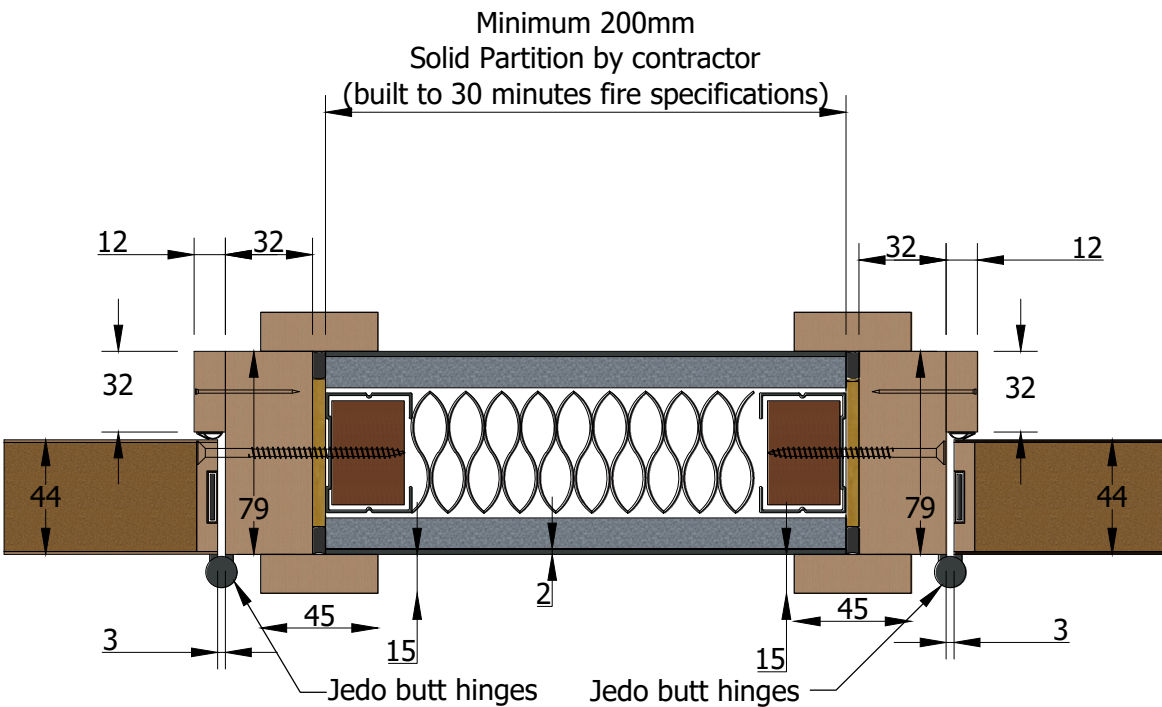
Detail D
