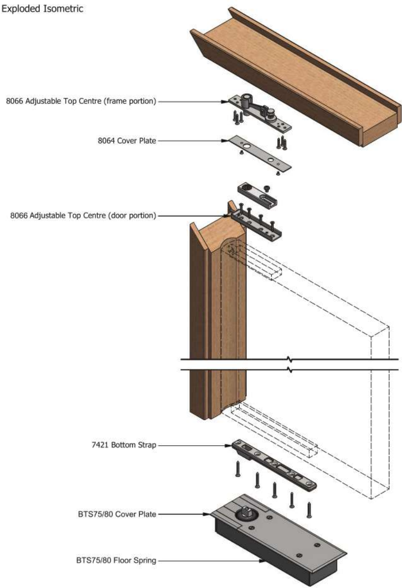
Exploded Isometric
