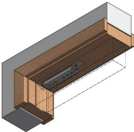
Isometric - Door Head
