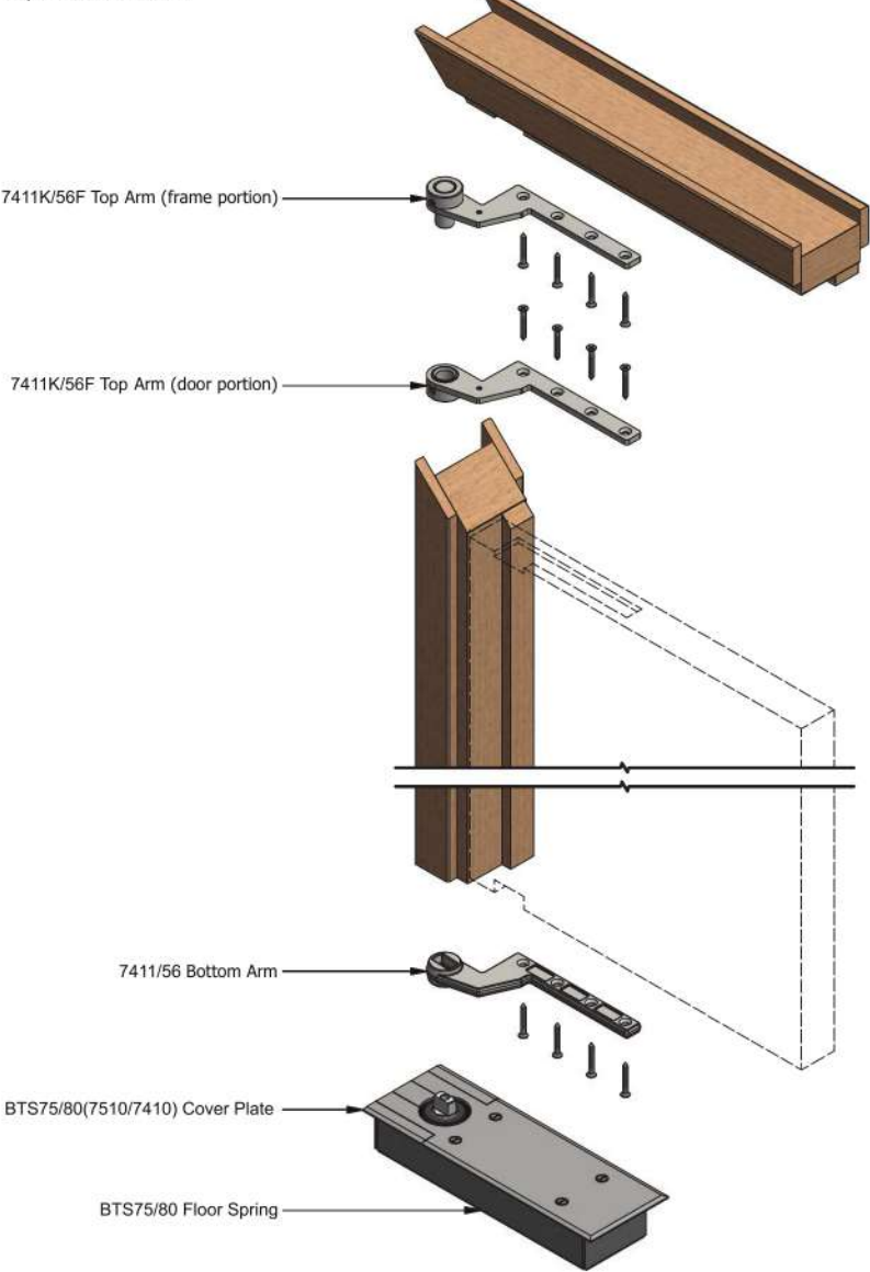
Exploded Isometric
