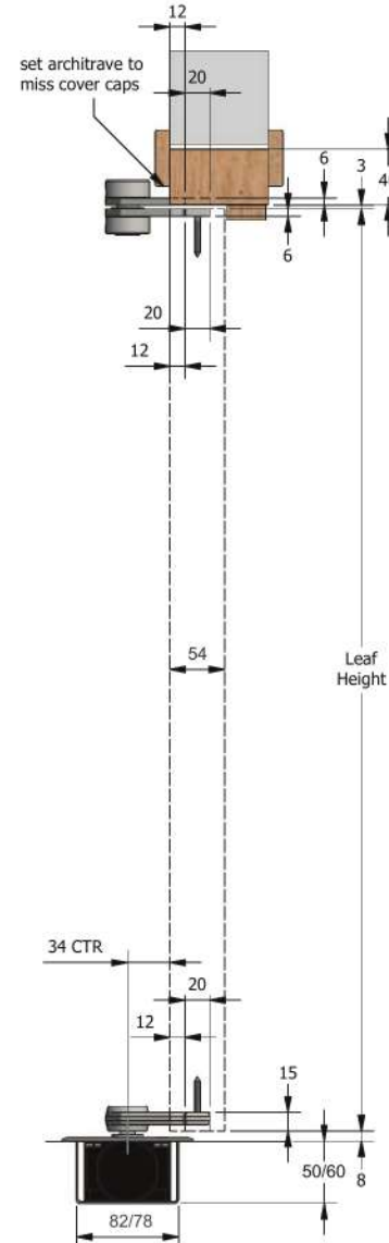
Vertical Section
