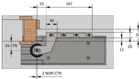
Plan Section (Door Base)
