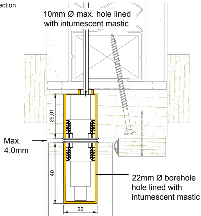
Section
