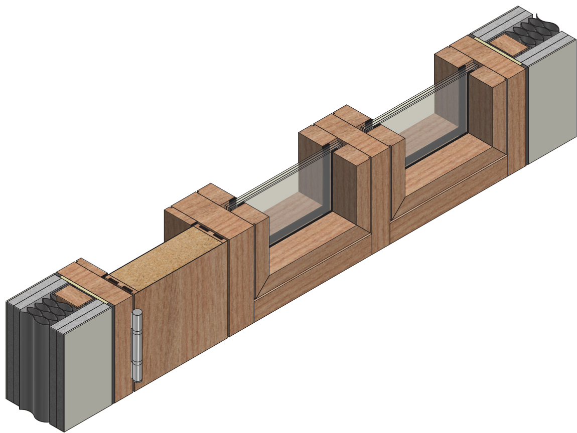
Isometric Timber/ Steel Stud FD60
