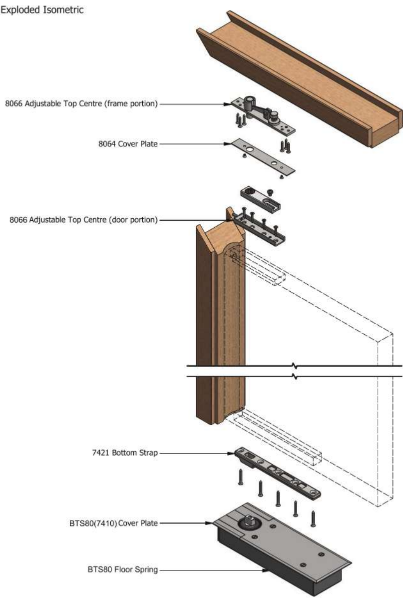
Exploded Isometric
