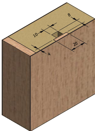
Concealed Cable-way in Door Leaf
