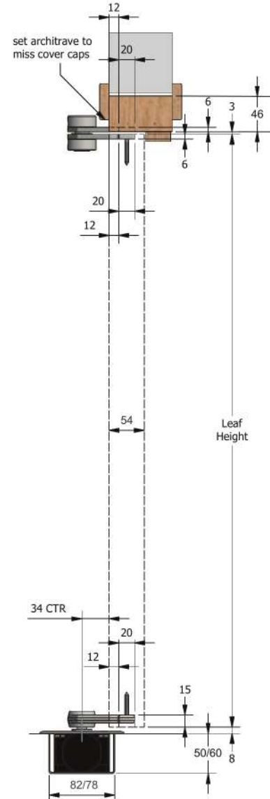
Vertical Section
