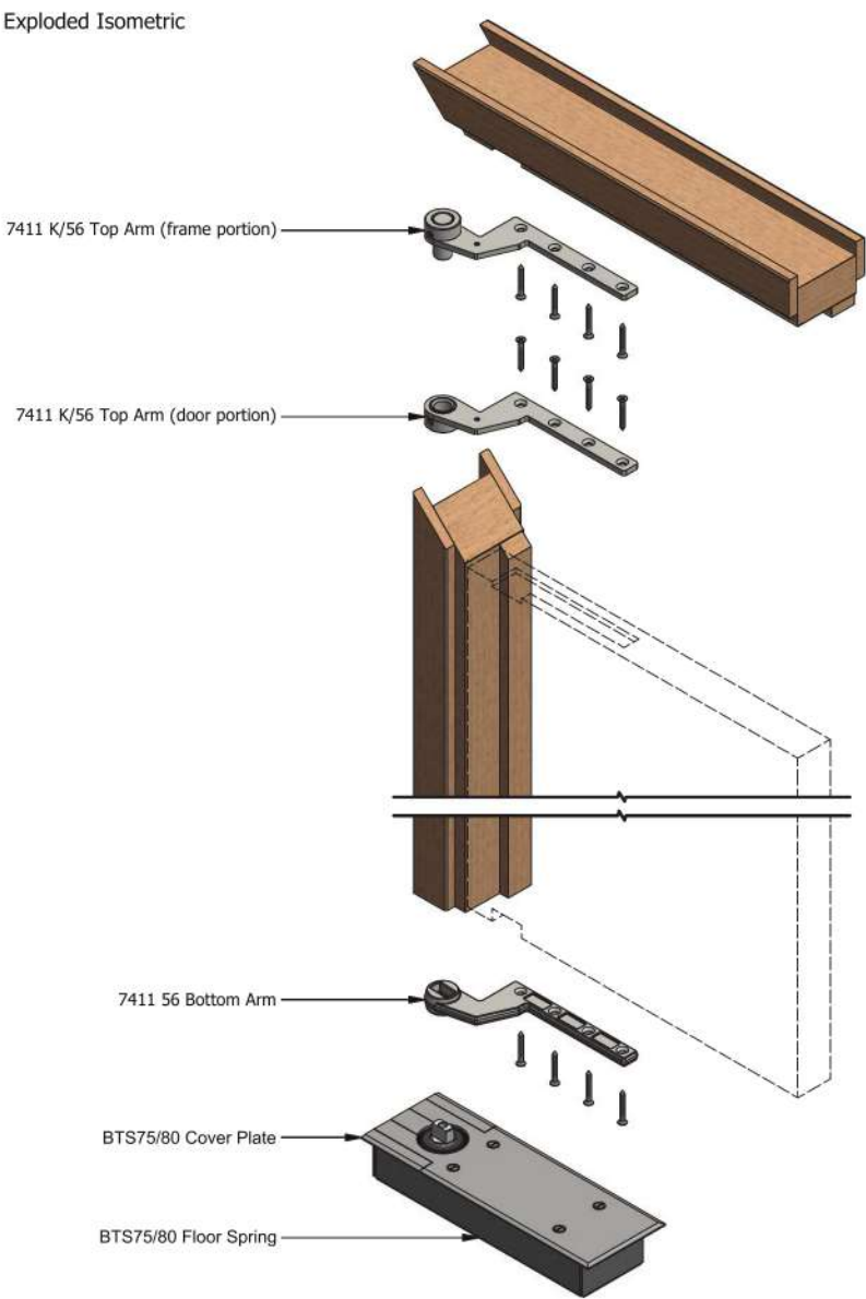
Exploded Isometric
