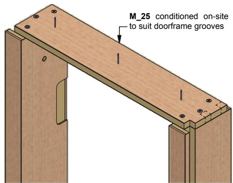
Doorframe Top Right Isometric
