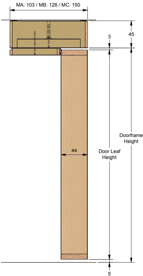
Head and Base (1:3)
