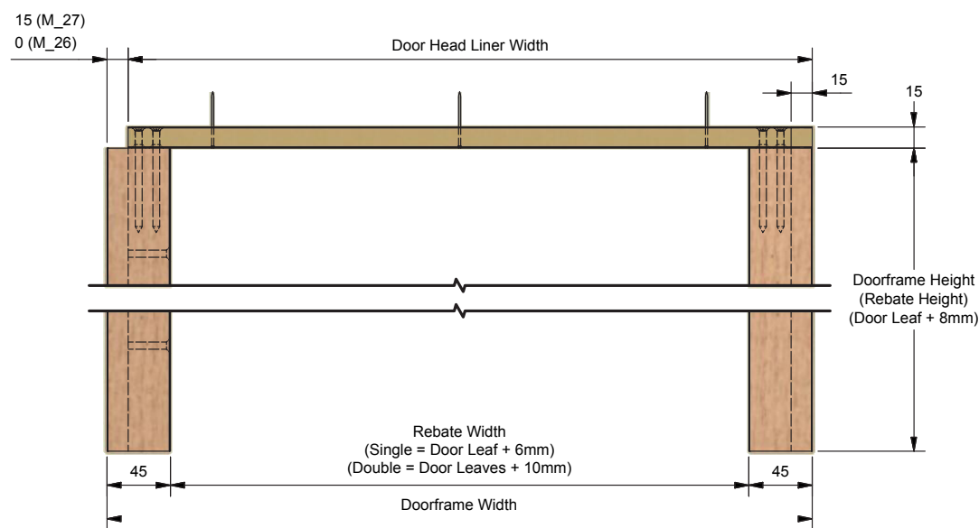
Doorframe Front View
